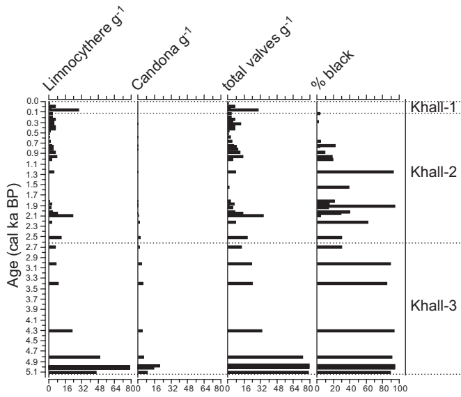
Fig. 4. Total ostracod concentrations (valves/g) are plotted on the calibrated age scale, along with the two most abundant genera Limmocythere sp. and Candona sp. The concentration of blackened valves is also given.
